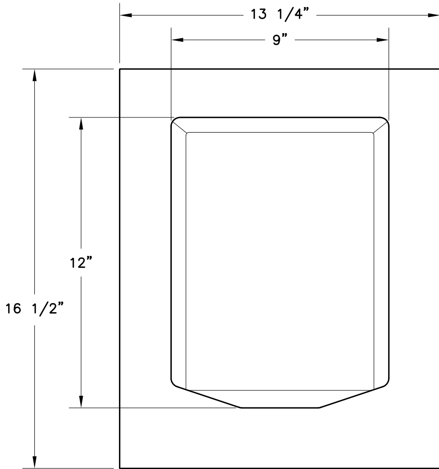
FRONT ELEVATION (MINUS DRAIN ADAPTER)
