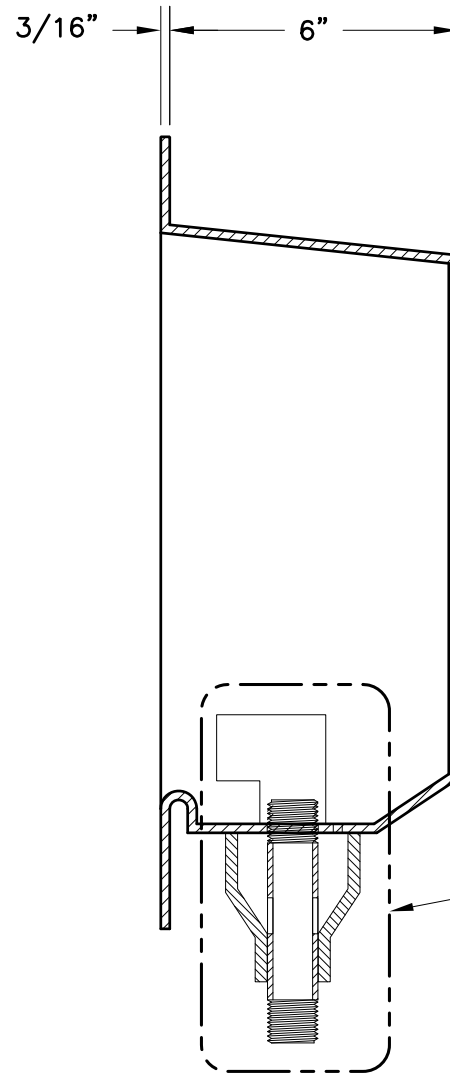
SECTION VIEW (WITH DRAIN ADAPTER)
